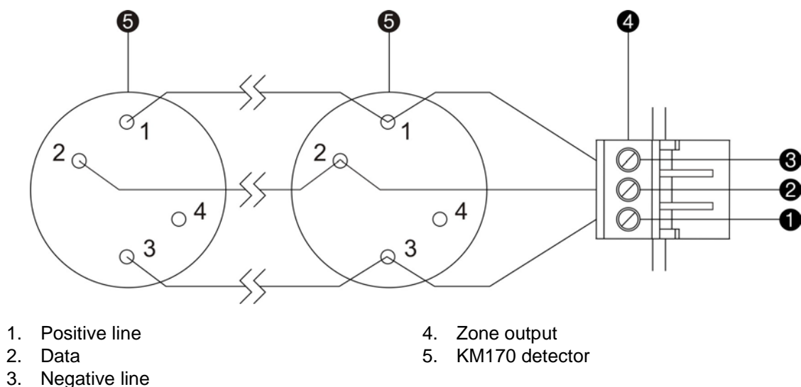
Figure 5: Zone line connection for KM170 detectors
